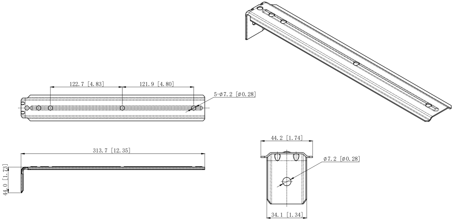
RIGHT VIEW 2:1
