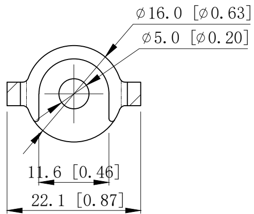
CUTAWAY VIEW A-A
