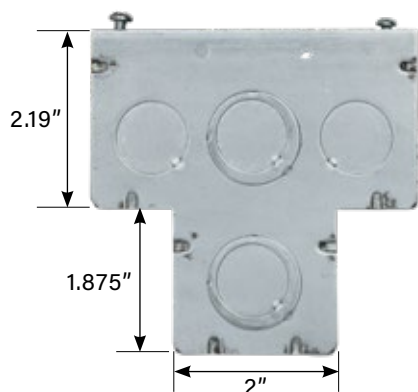
4" T Box
